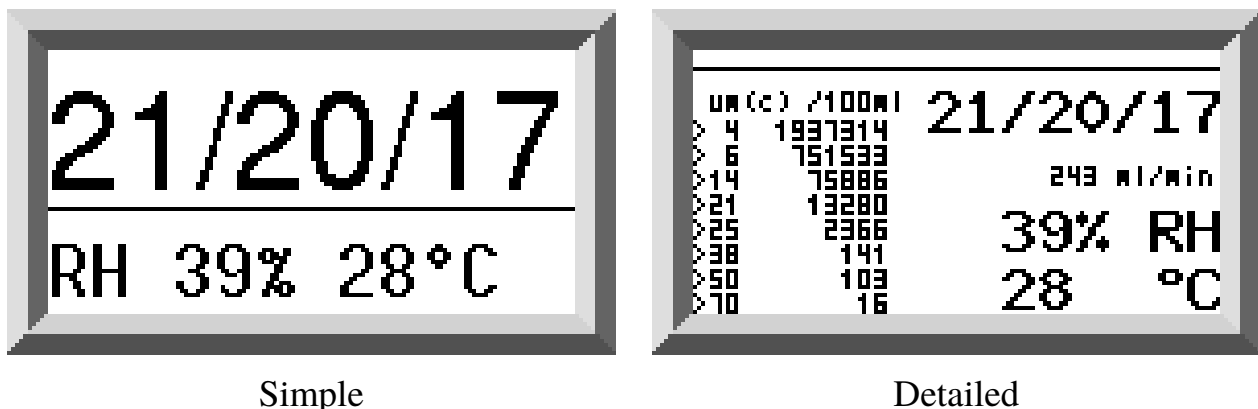
Figure 2 ISO4406:1999
